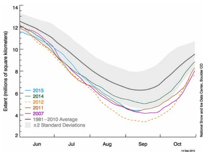
Figure 3: Graph showing the change in the Arctic sea ice extent (Image credit: NSIDC)
